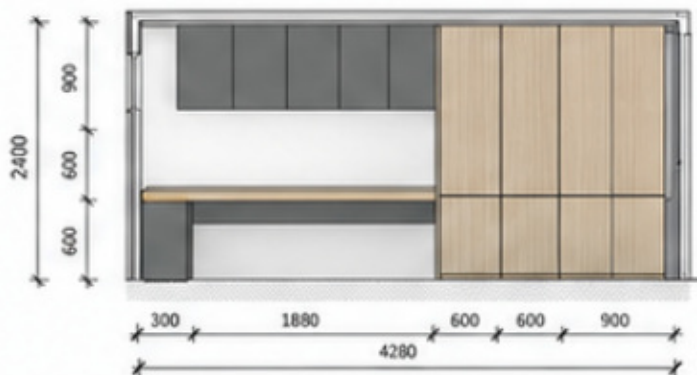
5 ELEVATION 1 - OFFICE JOINERY 1 : 50
