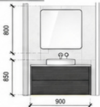
5 ELEVATION - ENSUITE 2 VANITY 1 : 20
