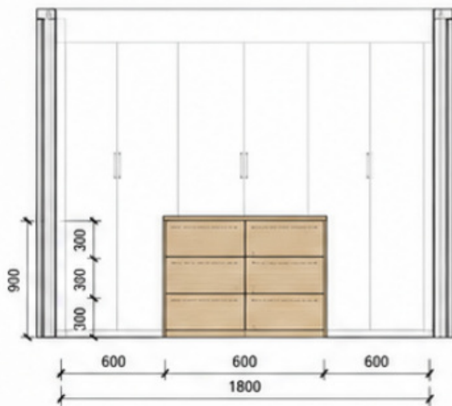
2 ELEVATION 1 - FRONT (ISLAND) 1 : 50
