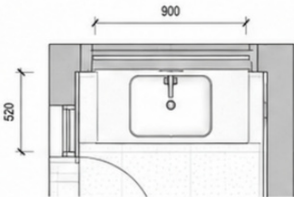
1 PLAN - BATH 1 VANITY 1 : 25
