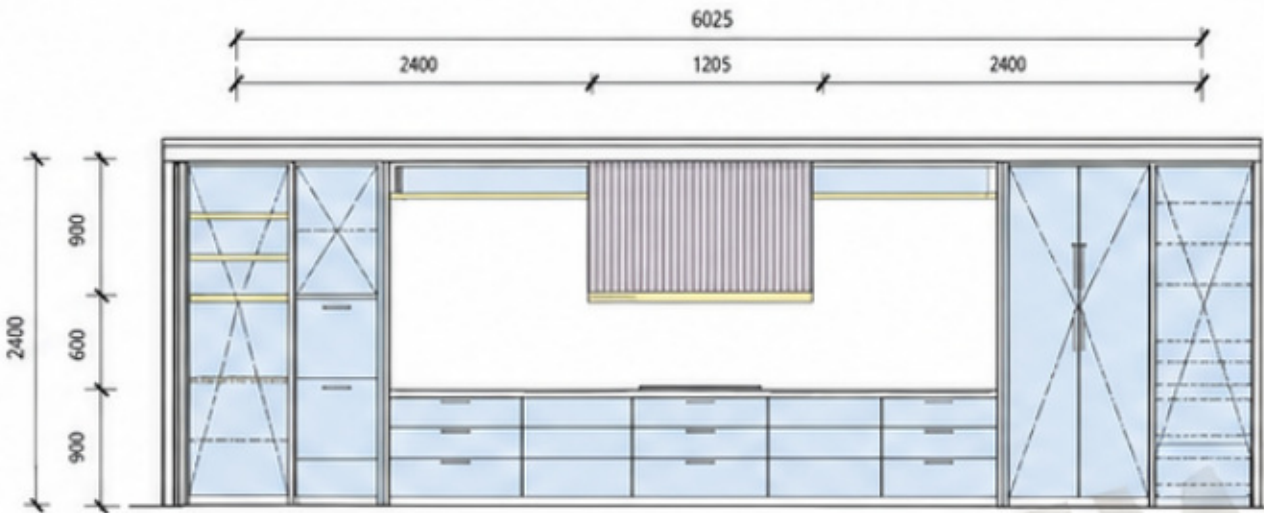
2 ELEVATION 1 - MAIN KITCHEN 1 : 50
