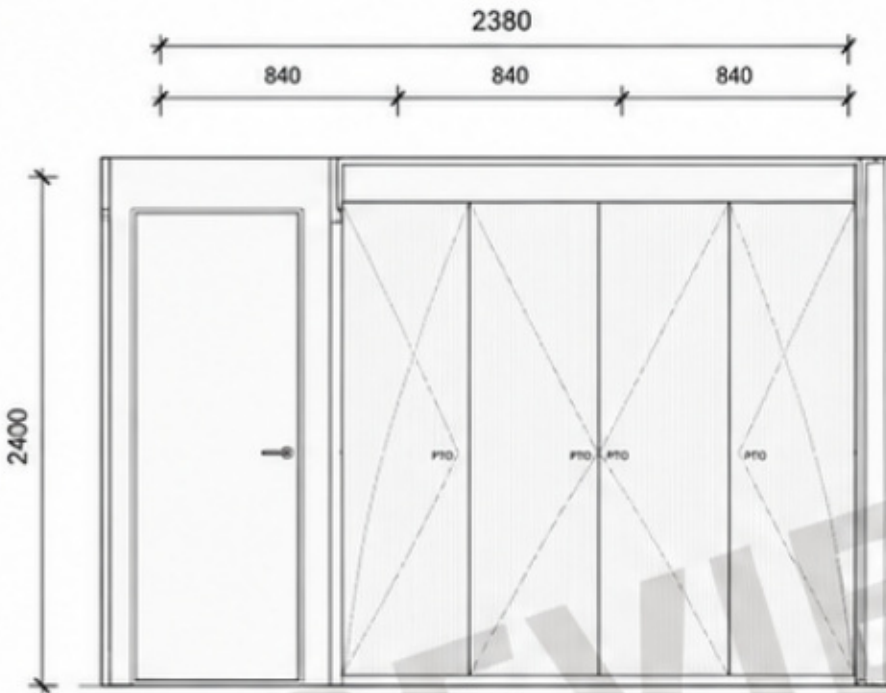
2 ELEVATION 1 - TALL STORAGE 1 : 50
