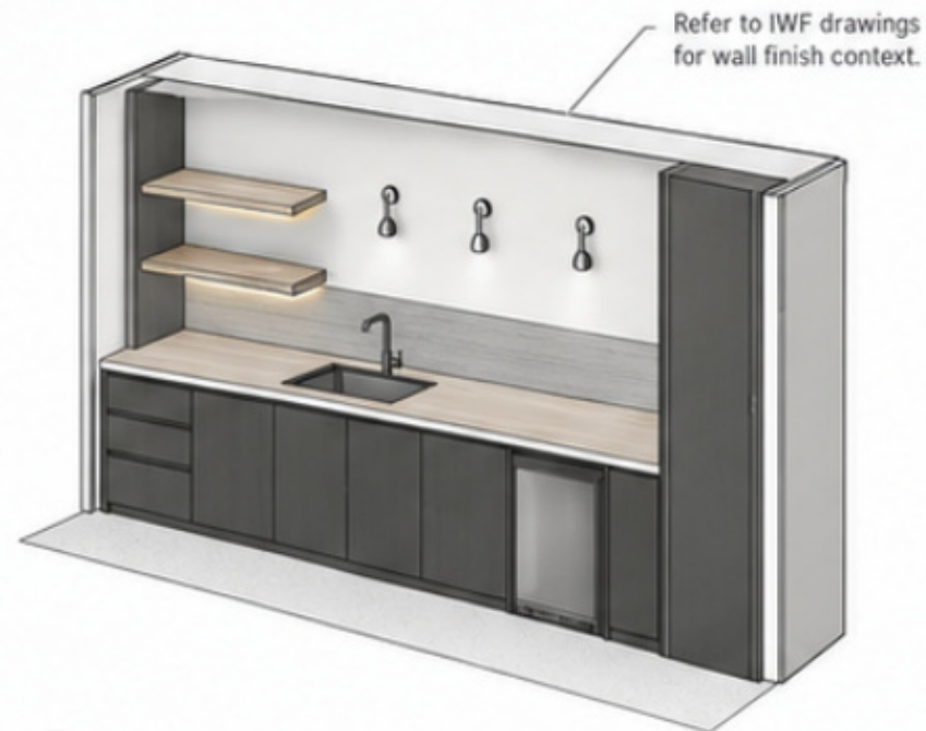
6 PERSPECTIVE VIEW - MEDIA KITCHENETTE NTS
