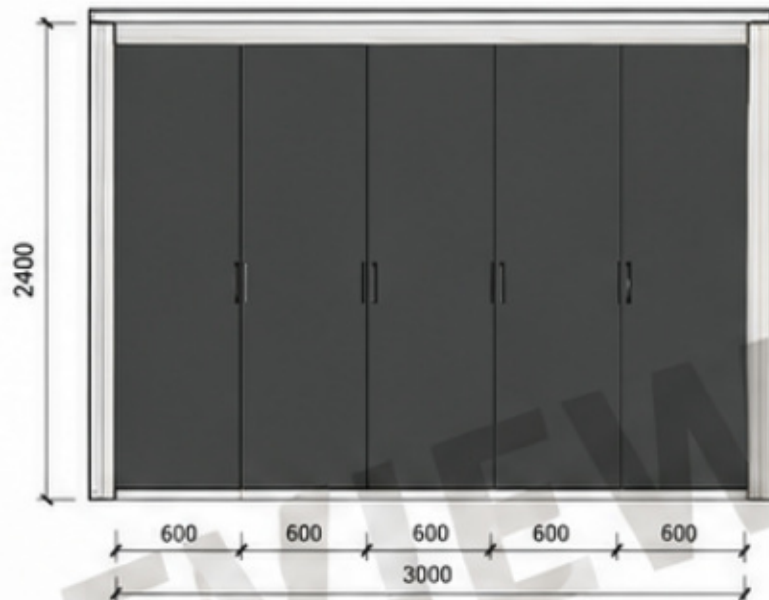
3 ELEVATION 2 - NORTH ROBE RUN 1 : 50
