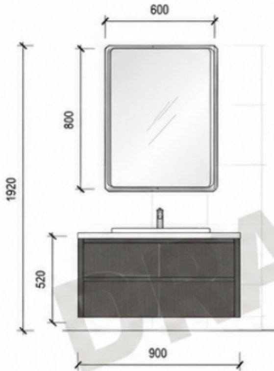
2 ELEVATION 1 - BATH 1 VANITY 1 : 25
