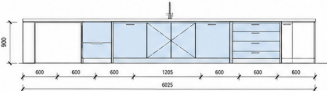
5 ELEVATION 4 - BACK OF ISLAND 1 : 50
