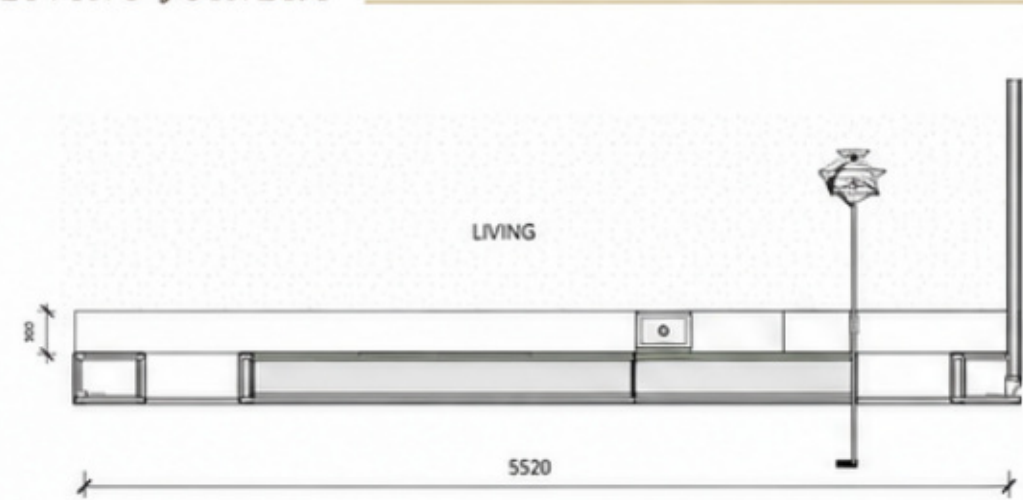
1 PLAN - LIVING JOINERY 1 : 50
