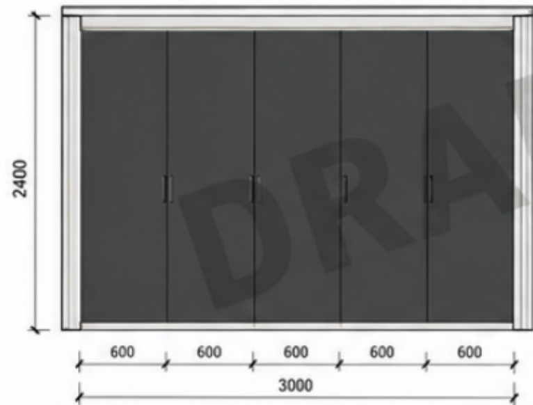
4 ELEVATION 3 - SOUTH ROBE RUN 1 : 50
