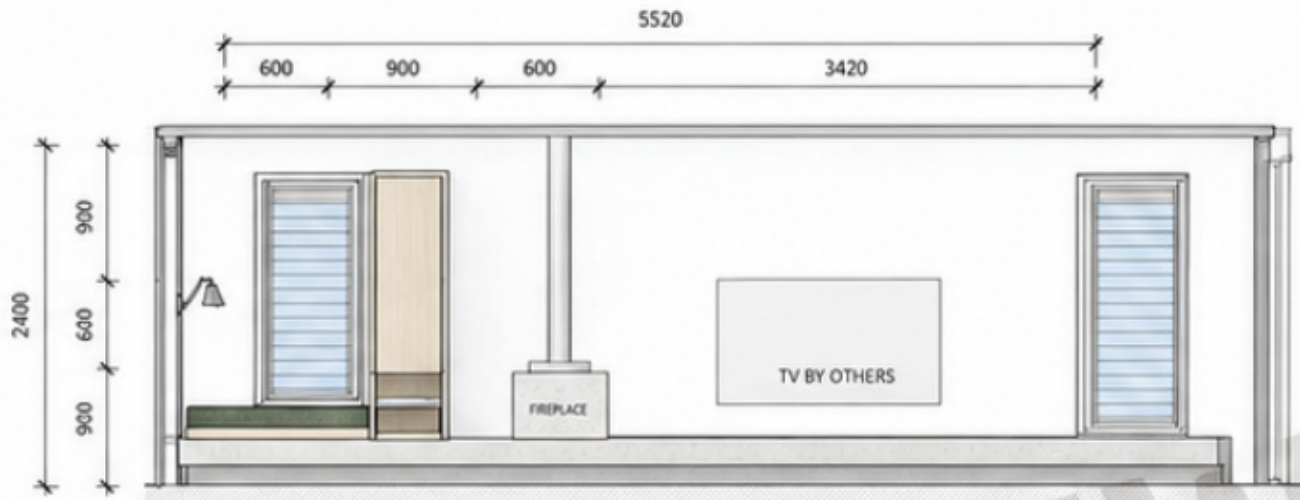
2 ELEVATION 1 - LIVING JOINERY 1 : 50
